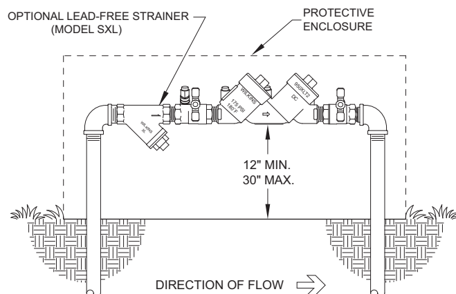
OUTDOOR INSTALLATION
