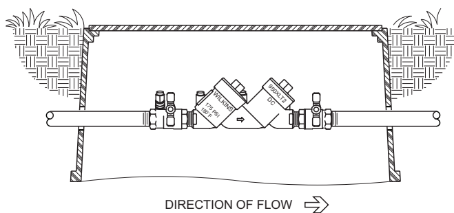
PIT INSTALLATION
